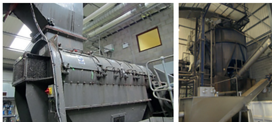
Figure 7: Left – Food de-packaging machine. Right – Linde hydropulper in operation at Valorsul AD plant (courtesy FP7 VALORGAS).
